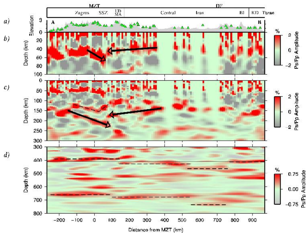
Figure 1. Depth migration of 246 P-receiver functions beneath Zagros profile ( x < 300 km) and NE Iran profile ( x > 300 km). Vectors mark rapid change of Moho boundary in front of MZT
