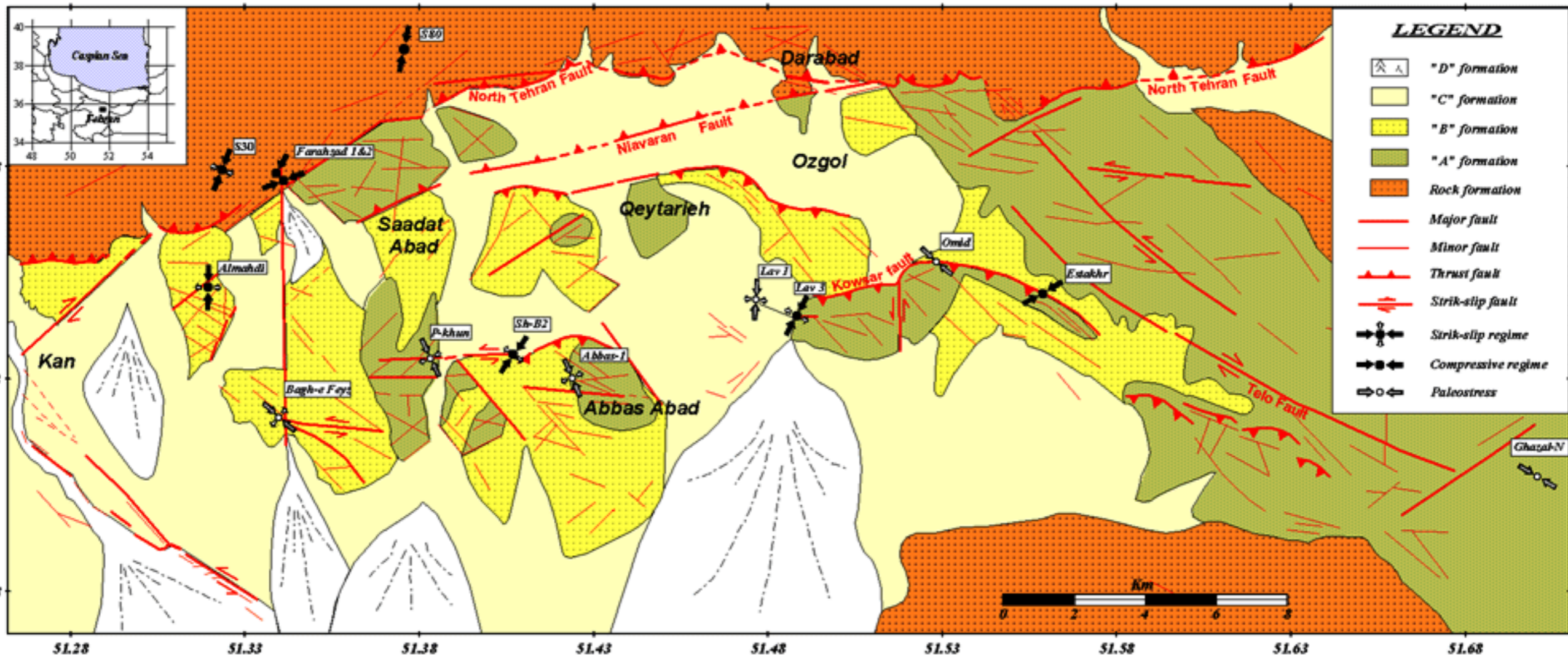
FAULT MAP OF NORTH TEHRAN (After Abbassi & Shabanian-B, 1999)
